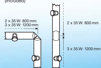
Typical installation with system end pieces
